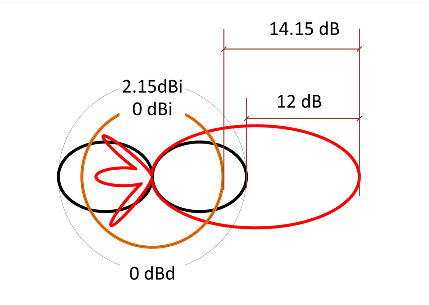
Figure 2. Adding dBi to our antenna comparisons
