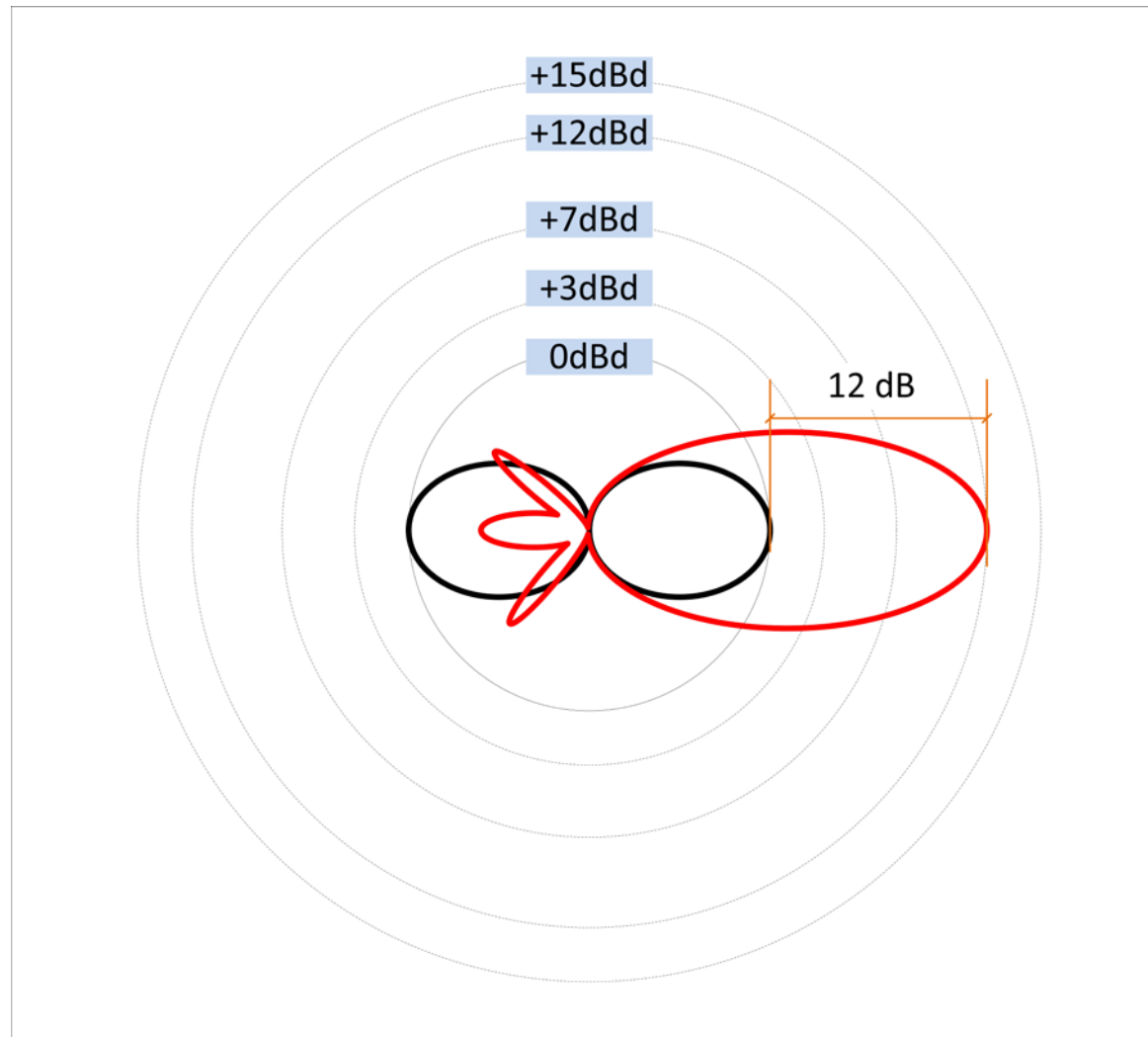
Figure 1. Comparison of antenna radiation patterns
