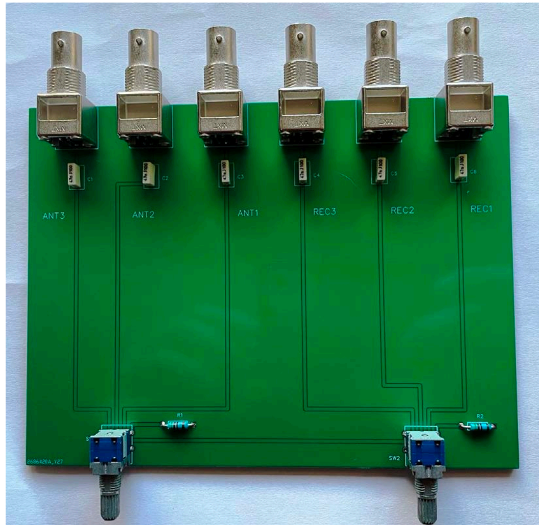
Figure 2. Top view of PCB
